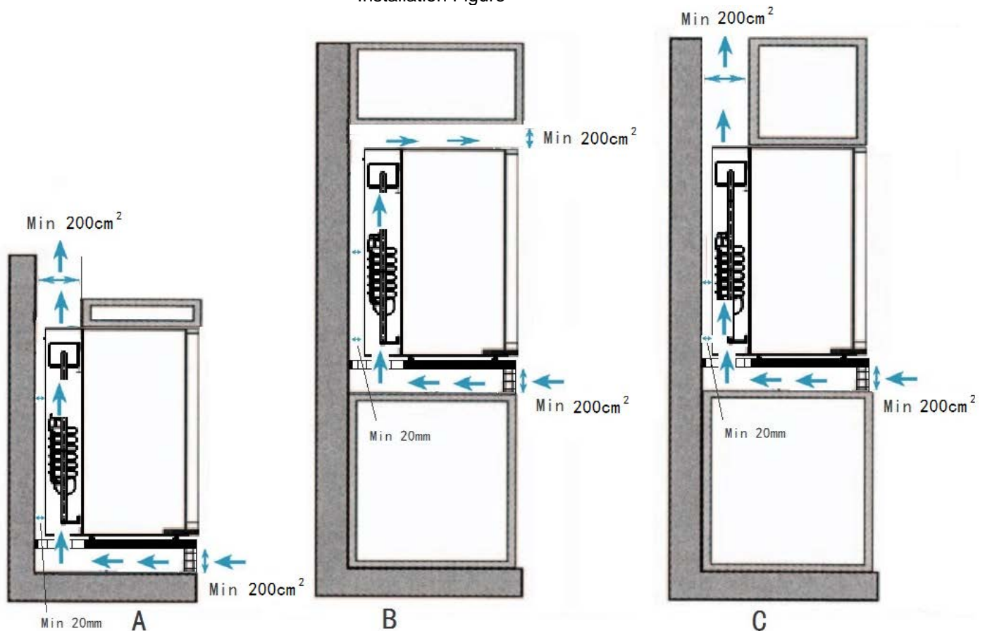
Installation Figure
